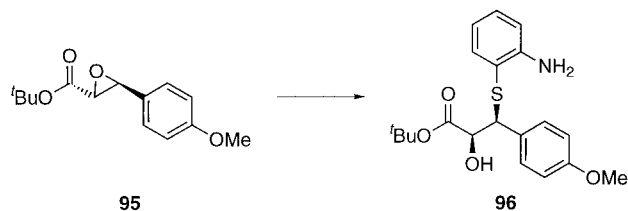
Scheme 15. Reagents and conditions: o -aminothiophenol, PhMe, 110°C, 90%.
