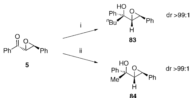
Scheme 10. Reagents and conditions: i. n -BuMgI, diethyl ether, -78^{\circ}\text{C} , 60%; ii. MeMgI, diethyl ether, -78^{\circ}\text{C} , 89%.
