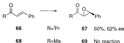
Scheme 9. Reagents and conditions: aq. H 2 O 2 , aq. NaOH, DCM, poly-L-leucine, 168 h.
