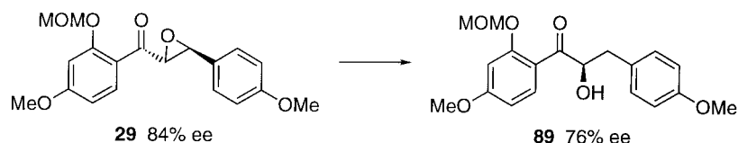
Scheme 12. Reagents and conditions: \text{H}_2 , Pd/BaSO 4 , MeOH, 88%.
