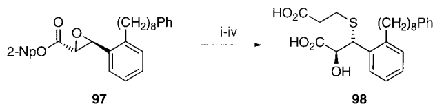
Scheme 16. Reagents and conditions: i. LiOH, H 2 , MeOH, 95%; ii. MeO 2 C(CH 2 ) 2 SH, NaOMe, THF, MeOH; iii. NaOH, H 2 O; iv. HCl, H 2 O, 76%.
