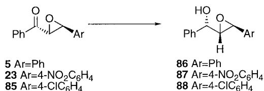
Scheme 11. Reagents and conditions: \text{Zn}(\text{BH}_4)_2 , \text{Et}_2\text{O} , 0^{\circ}\text{C} , 100%.
