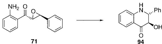
Scheme 14. Reagents and conditions: n -butanol, 85°C, 64%.
