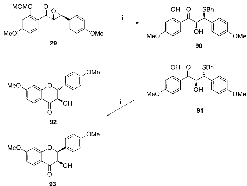
Scheme 13. Reagents and conditions: i. BnSH, SnCl 4 , DCM, -20 to 0°C, 93%; ii. AgBF 4 , DCM, 71%.
